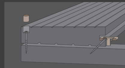
Spezial-Clip Special clip
